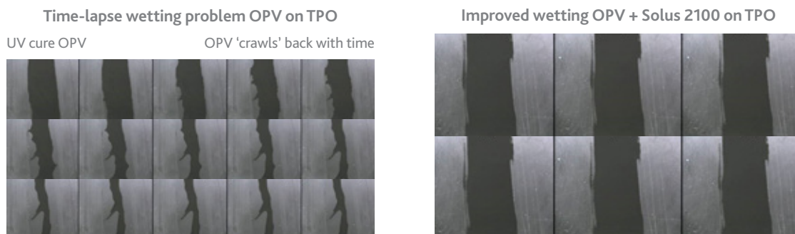
Figure 10. Wetting and crawl of an acrylate OPV without and with Solus 2100
