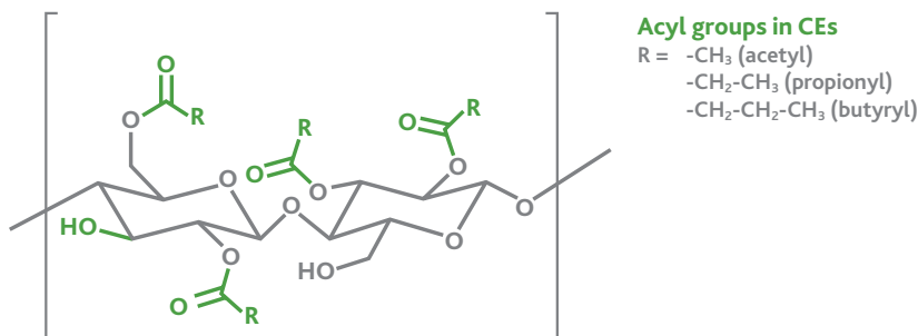
Figure 2. Chemical structures of cellulose esters
