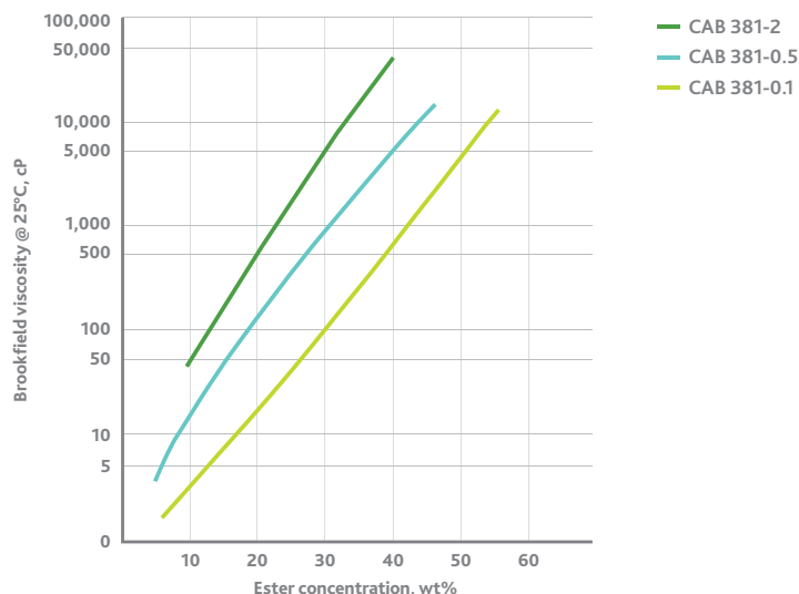
Figure 4. Impact of molecular weight on Brookfield viscosity
